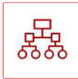
Image Classification
